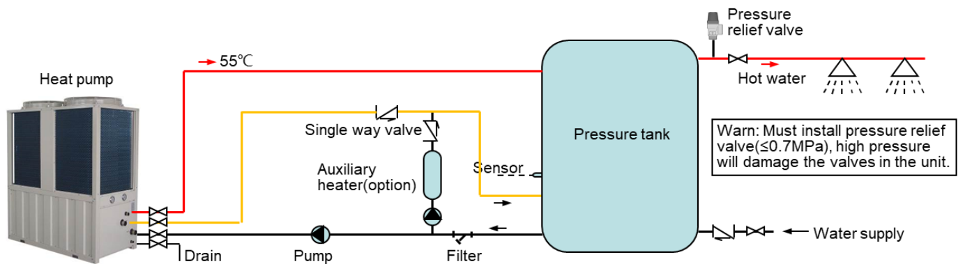
Diagram 2 — Hot water system(with auxiliary heater)
