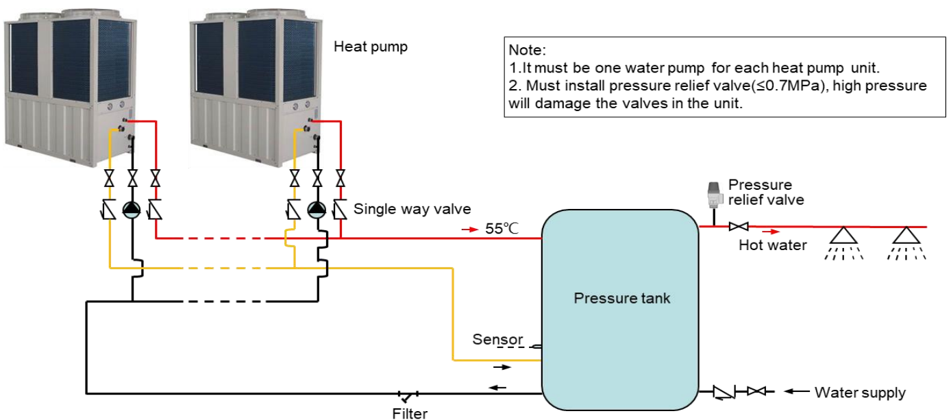
Diagram 3 — Modular hot water system
